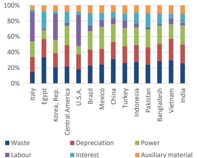
Figure 2: Manufacturing cost for spinning Ring/NE30 (USD/Kg)
