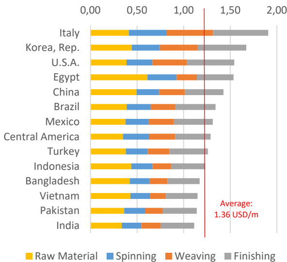
Figure 1: Total cost of producing a finished meter of woven fabric (CO, COW), by segment (USD/m)
